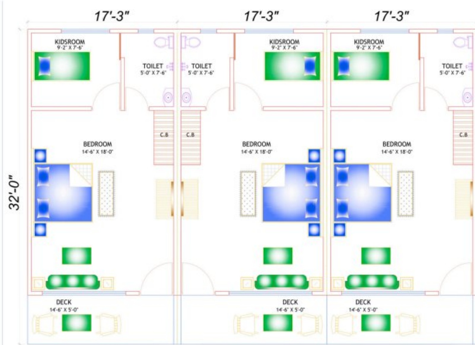
1BHK COTTAGE UNIT PLAN
