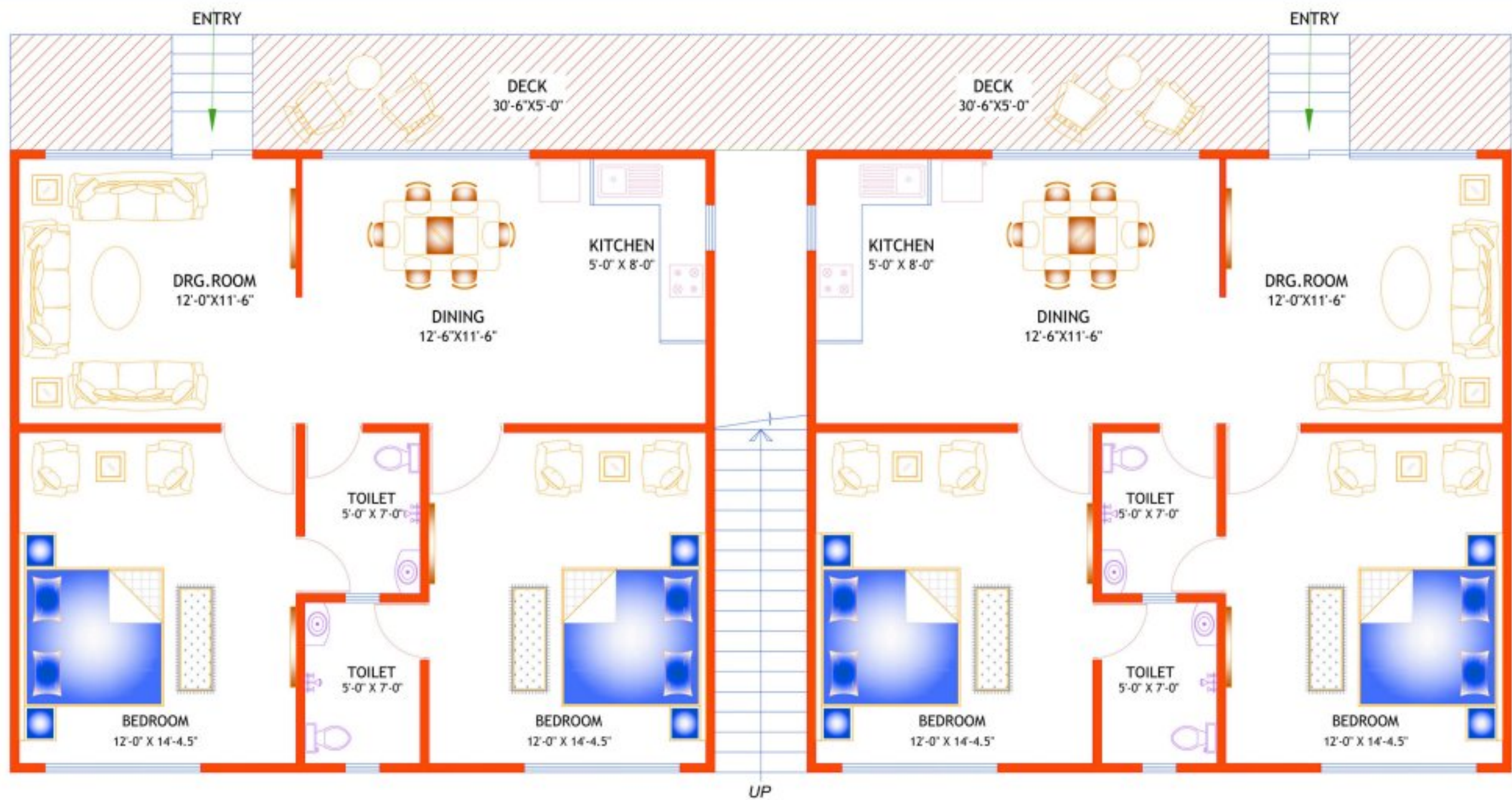
2BHK GROUND FLOOR UNIT PLAN
