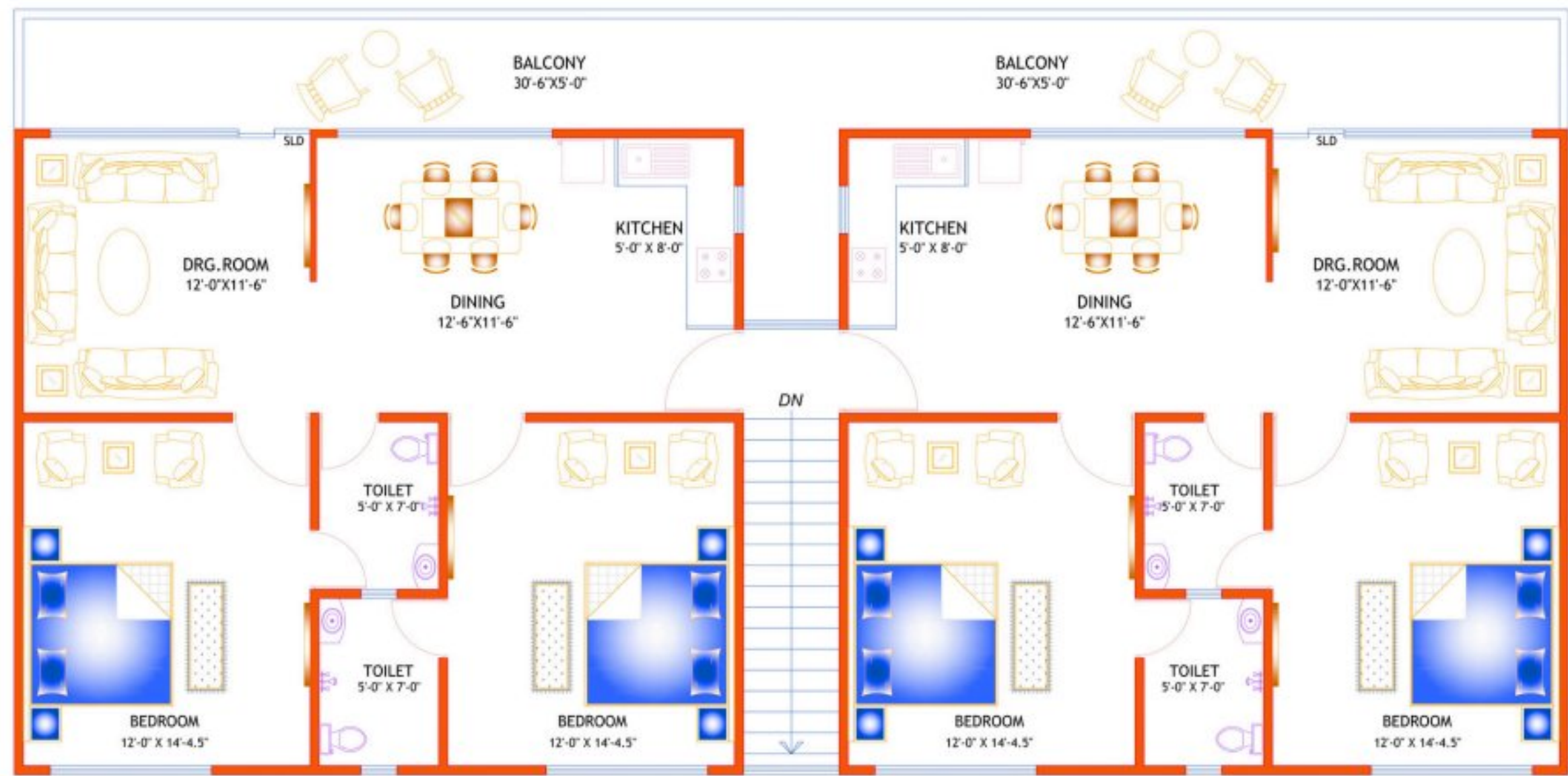
2BHK FIRST FLOOR UNIT PLAN
